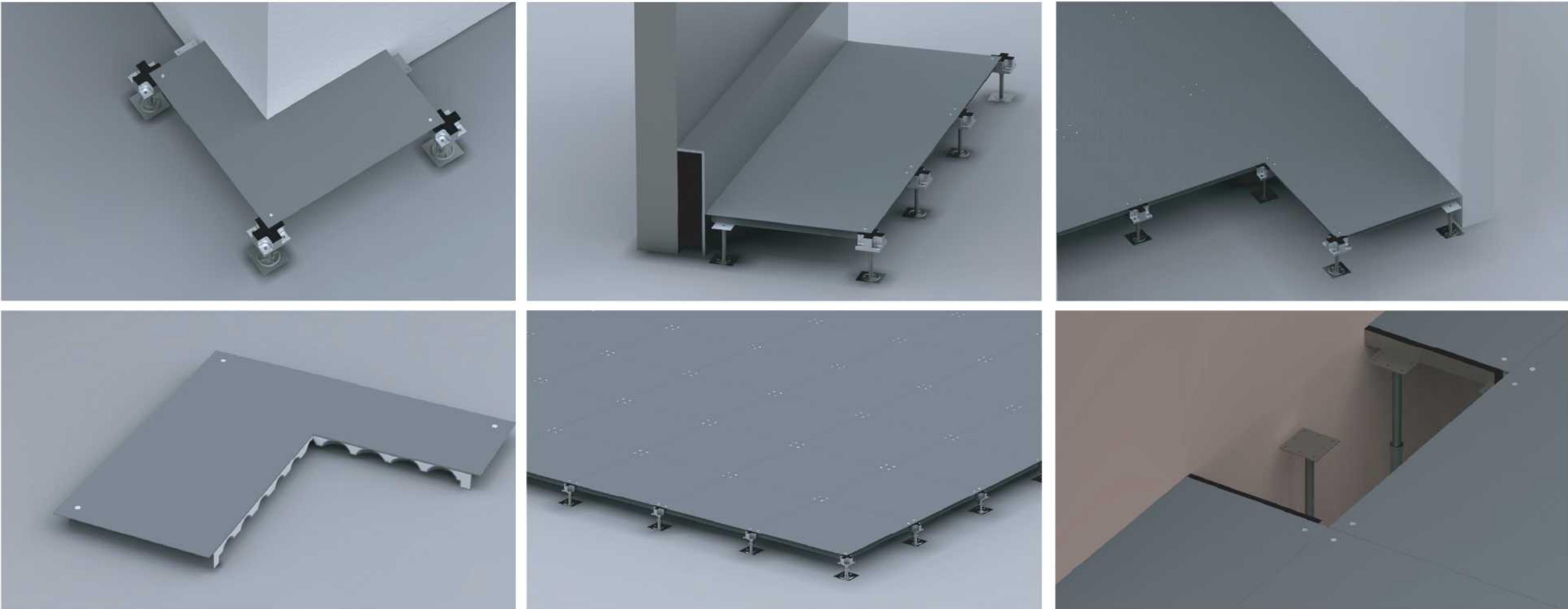
OA地板节点安装示意图 OA SERIES INSTALLATION DRAWINGS
