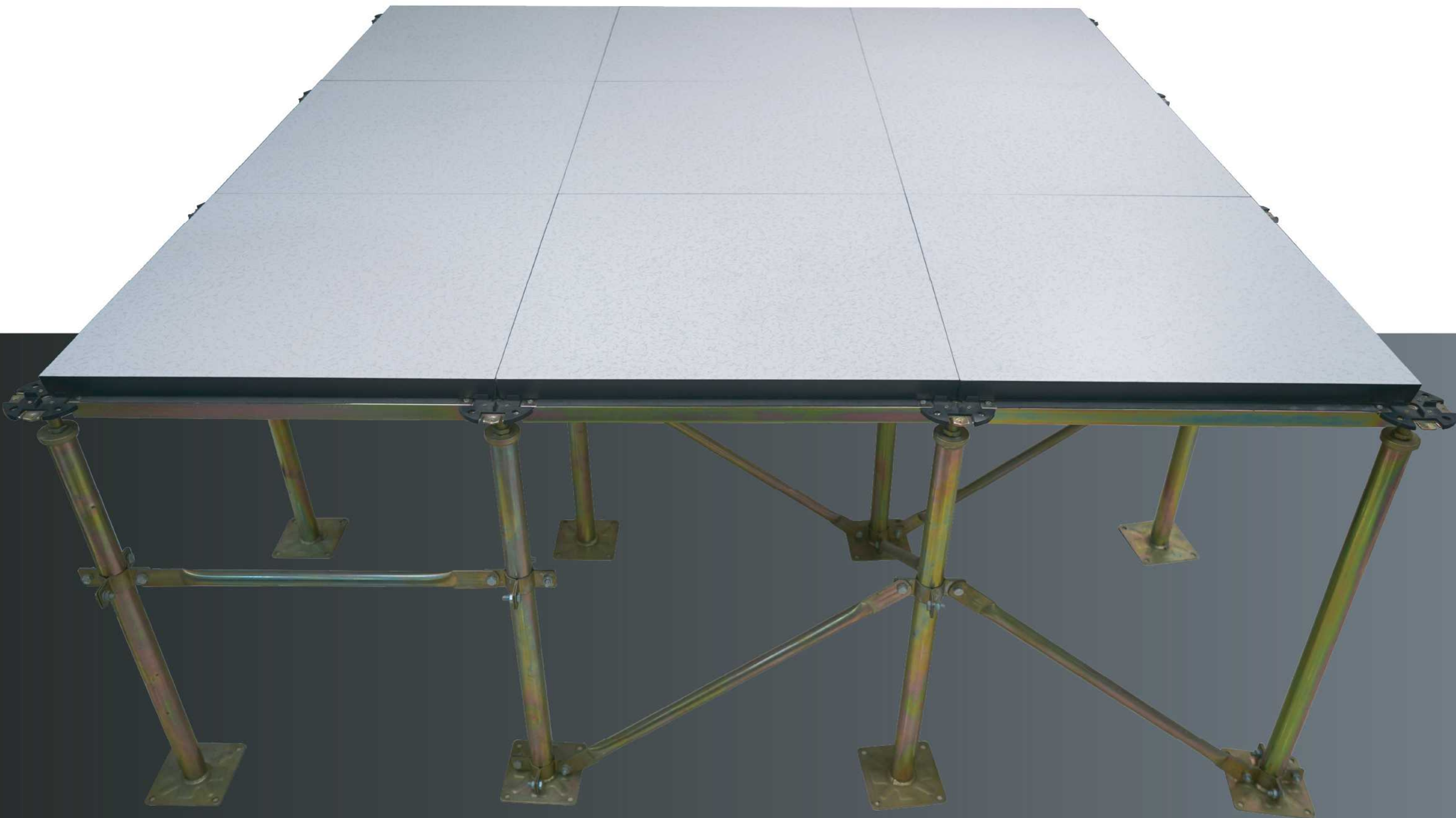
铺装效果图 EFFECT DRAWING OF PAVEMENT
